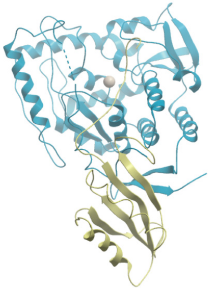
mouse PAH (1phz)
